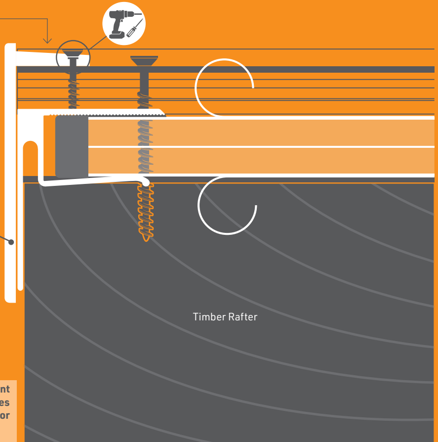
SECTION DETAIL
