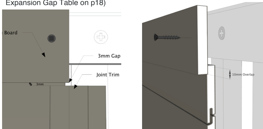
3mm* gap between Board & Trim
