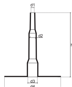
CONNECTOR
